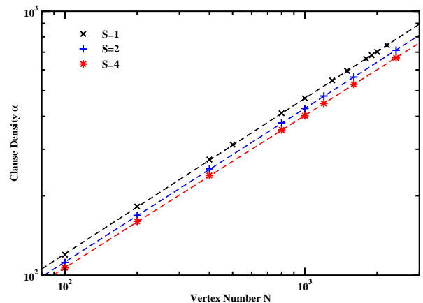
FIG. 7: (color online). Scaling behavior between variable number N and the characteristic clause density \alpha = \alpha_0 of the focused local search algorithm. The control parameter of the focused local search algorithm is S . The dashed lines are fitting curves of the form \alpha_0 = c \times N^b . The fitting parameters are c = 8.0 \pm 0.1 and b = 0.589 \pm 0.002 (top, S = 1 ); c = 7.7 \pm 0.1 and b = 0.582 \pm 0.002 (middle, S = 2 ); and c = 7.5 \pm 0.1 and b = 0.577 \pm 0.002 (bottom, S = 4 ).
