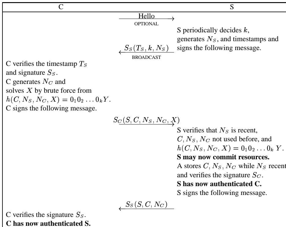
Fig. 2. DOS-resistant authentication with public-key signatures
