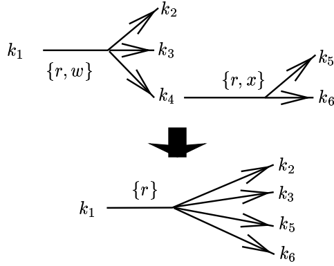
Figure 4: Certificate reduction
