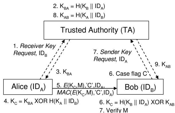
Figure 4 Combined Sender and Receiver ID Based AKE
