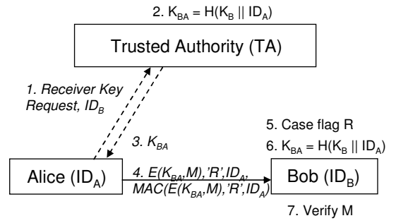
Figure 3: Receiver ID-Based AKE
