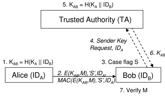
Figure 2: Sender ID-Based AKE
