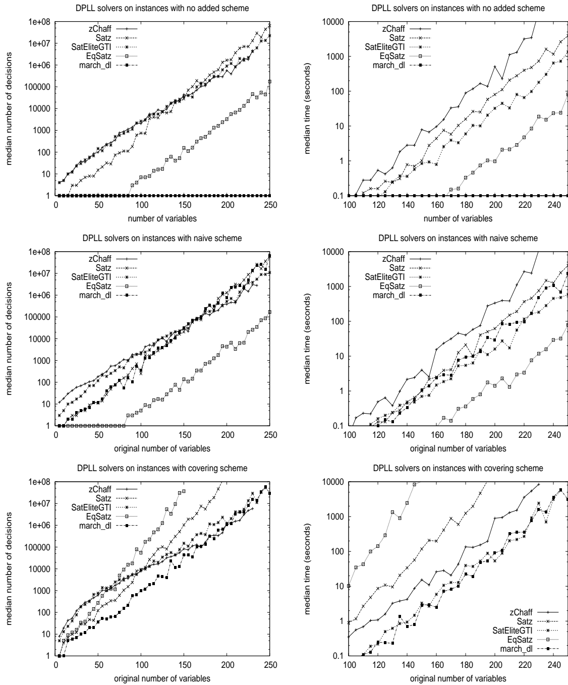
Figure 7. Comparison of different solvers against added nonlinearity: median number of decision (left) and median running times (right), with no added nonlinearity (top), with the naive scheme (middle), and with the covering scheme (bottom).
