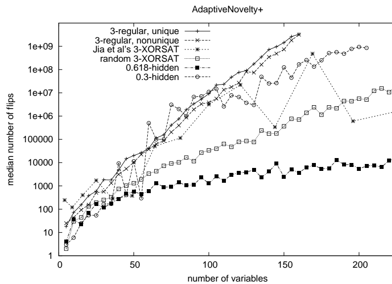
Figure 6. Hard satisfiable instance families for local search: median of number of flips as reported by AdaptiveNovelty+.
